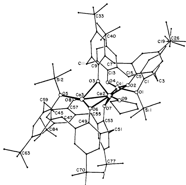
Figure 4. Computer-generated drawing of the skeleton of 4 (no hydrogen atoms or toluene molecules have been included).
