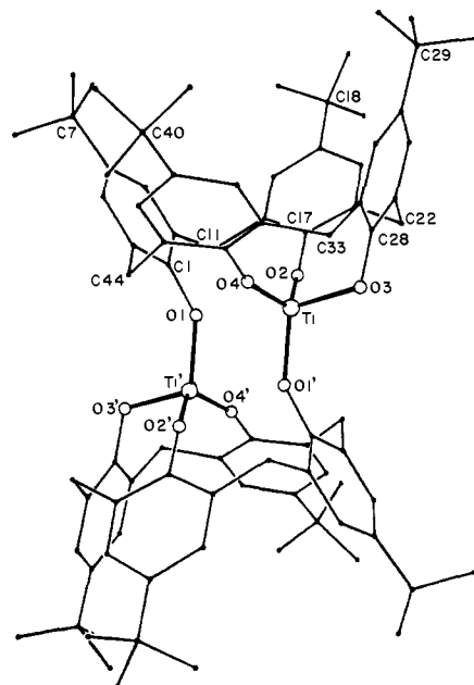
Figure 2. Computer-generated drawing of the skeleton of 2 (no hydrogen atoms or toluene molecules are shown).
