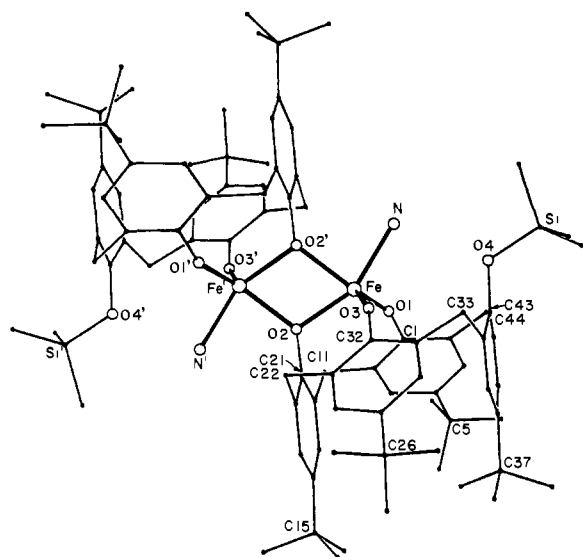
Figure 3. Computer-generated drawing of the skeleton of 3 (no hydrogen atoms or hexane molecules are shown).
