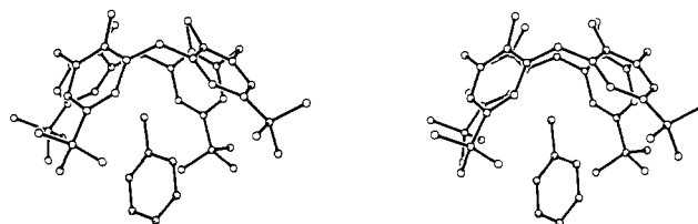
Figure 5. Stereoview of one of the ligands in 4 showing the interaction of a toluene with the calixarene.
