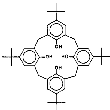
Figure 1. Representative drawing of ligand 1.
